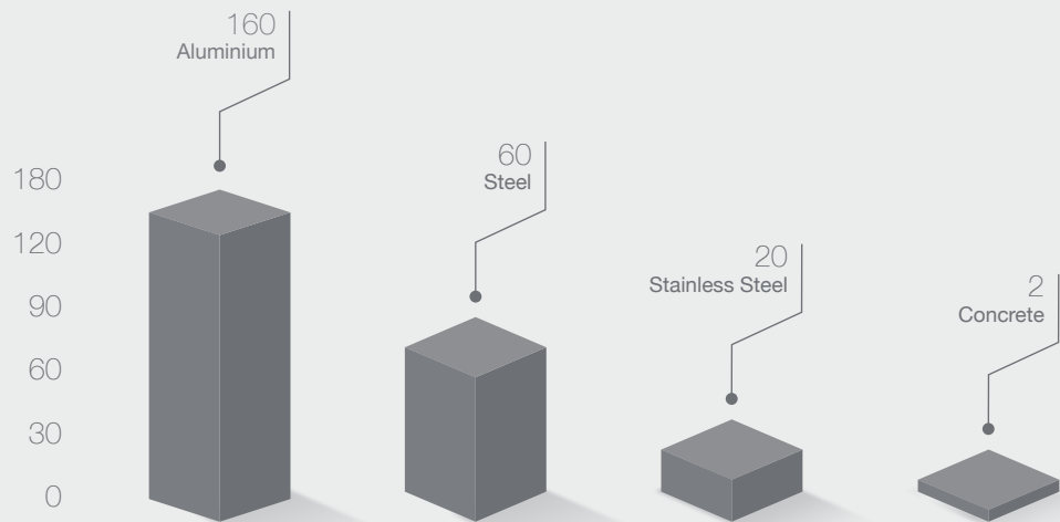
Thermal conductivity values of Armatherm™ structural thermal break materials as compared to standard building materials.
